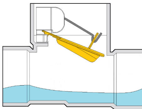
Normally Open Normal Flow →
