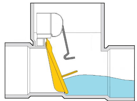
Closed Position * operates as check valve until reset
