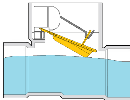
Gate Releases and Closes Reversal Flow ←
